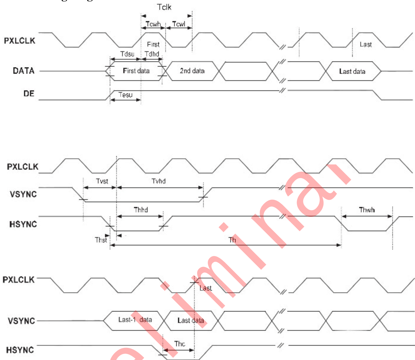
Clock and Data Input Timing Diagram
